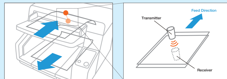
The sensor detect double-feeding and stops the scanner immediately. The high-performance sensor catches even subtle changes.
